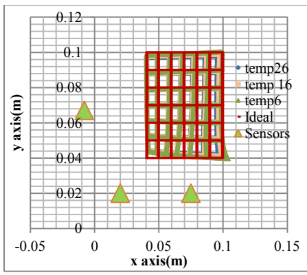
Figure 13: Temperature mismatch
