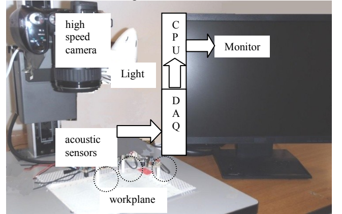
Figure 7: Hardware setup
