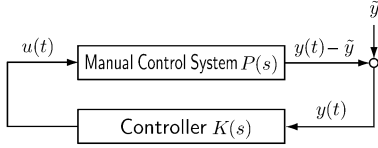
Fig. 2. Closed-loop system of the linearized system P(s) around the unknown operating point \tilde{y} in the manual control system and the proposed operator-support controller K(s) .
