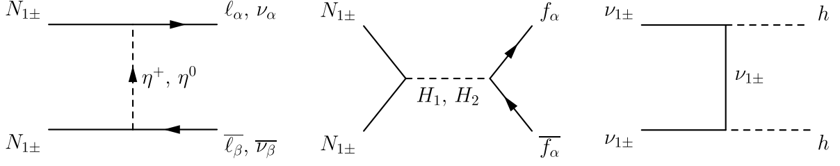
Figure 3: t , u and s -channel of coannihilation processes of DM \nu_{1\pm} .
