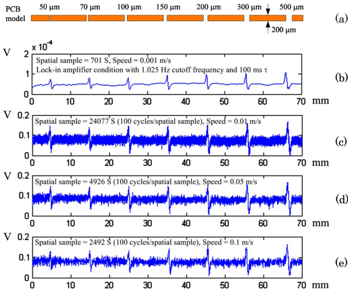
Fig. 7. Effect of scanning speed increasing. (a) PCB model, (b) ECT signal obtained from lock-in amplifier, and (c)–(e) ECT signal acquired by the proposed technique, with the number of samples of captured signal m of 100 cycles, at scanning speed of 0.01, 0.05, and 0.1 m/s, respectively.
