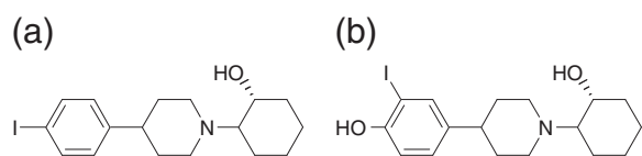
Figure 1 Chemical structures of (a) (+)- p IV and (b) (+)-IV-OH.
