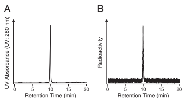
Figure 2 RP-HPLC chromatograms of (A) nonradioactive (+)-IV-OH and (B) (+)-[ 125 I] IV-OH after purification. Condition: flow rate was 1 mL/min. Mobile phase A was water with 0.1% triethylamine, and phase B was methanol with 0.1% triethylamine. The gradient conditions are as follows: 0 to 10 min, 70% to 80% B; 10 to 11 min, 80% to 100% B; and 11 to 20 min, 100% B.
