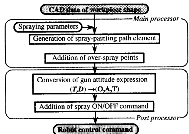
Fig. 5 Outline of spraying path generation
