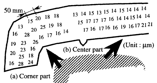
Fig. 10 Distribution of paint thickness
