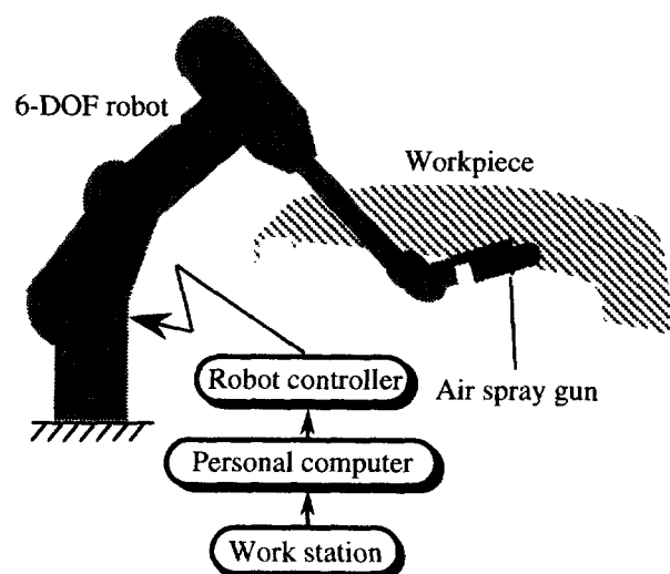
Fig. 1 Configuration of the spray-painting system
