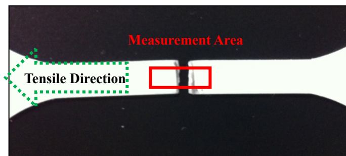
Fig. 9. Broken aluminum plate.
