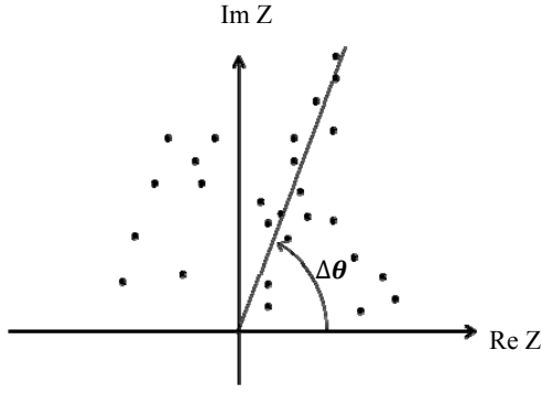
Fig. 4. Upper half complex plane plot of Z = [I_{\max}(\mathbf{r}) - I_{\min}(\mathbf{r})]\exp[i\delta(\mathbf{r}, t)] . \Delta\theta is the phase of the average value for [I_{\max}(\mathbf{r}) - I_{\min}(\mathbf{r})]\{\exp[i\delta(\mathbf{r}, t)] - (2/\pi)i\} . The number of points is 50, and one point overlaps
