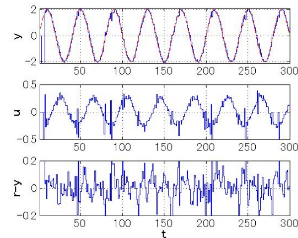
Figure 4 Simulation result of the linear system (17) when n=4 , m=2 , h=2 and k=10
