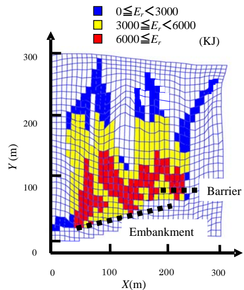
Fig. 12. Hazard map of rockfall.
