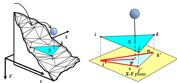
Fig. 3. Modeling of a slope as an assembly of triangle planes and a projected triangle plane to X-Y plane under the rock.
