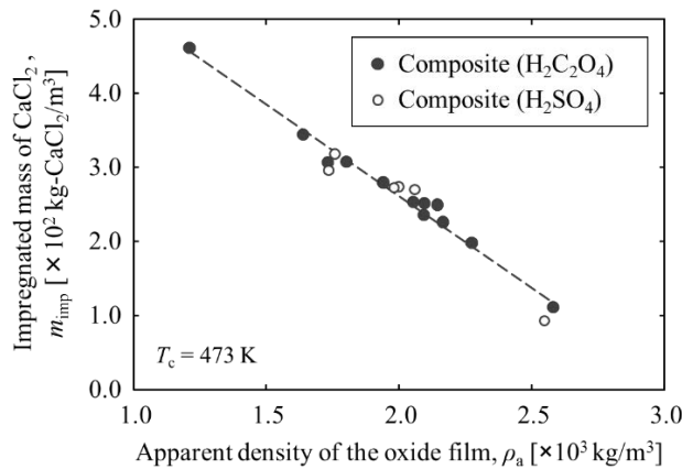
Fig. 1 Relationship between impregnated mass of CaCl 2 onto anodic alumina film and apparent density of the film.
