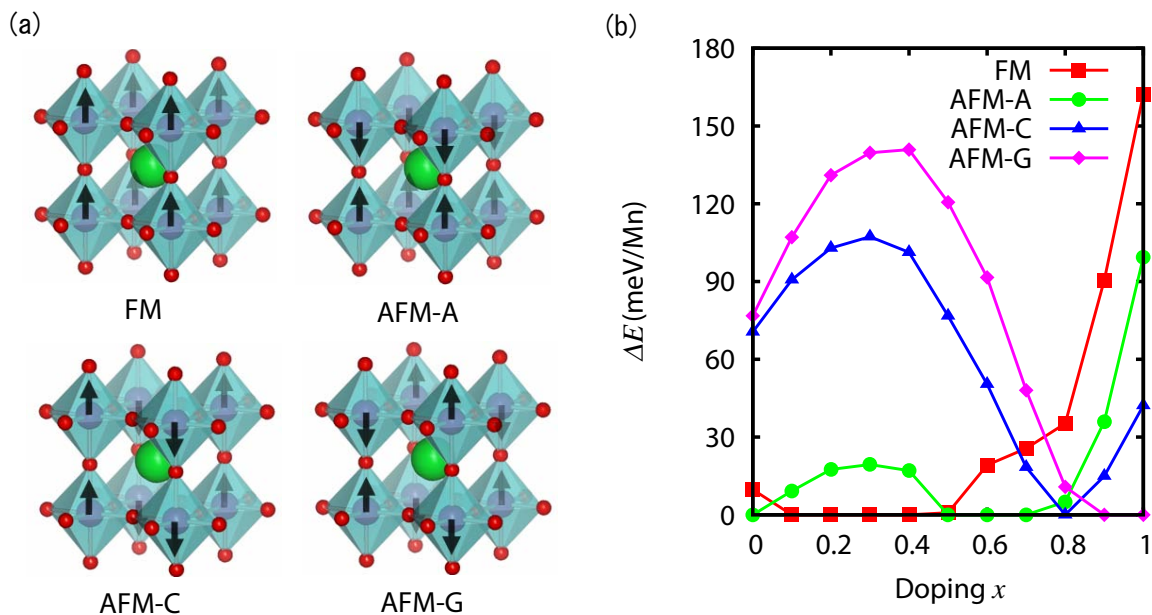
Figure 1. (a) The collinear magnetic structures of \text{La}_{1-x}\text{Sr}_x\text{MnO}_3 . (b) The total energy difference per Mn atom from the stable state as a function of x . The red squares, green circles, blue triangles and pink diamonds denote the FM, AFM-A, AFM-C and AFM-G states, respectively. The lines serve as a visual reference.
