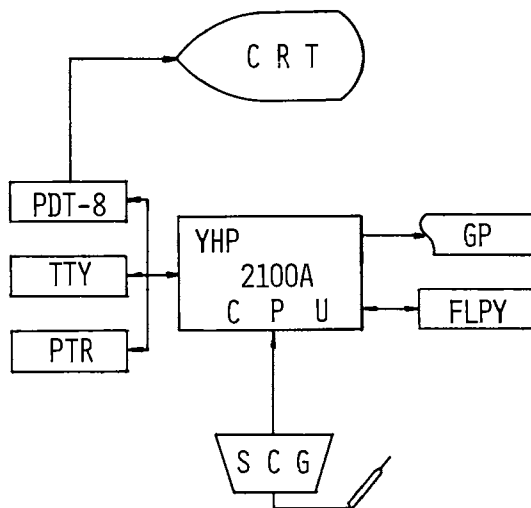
Fig. 4 Hardware System of VISMS
