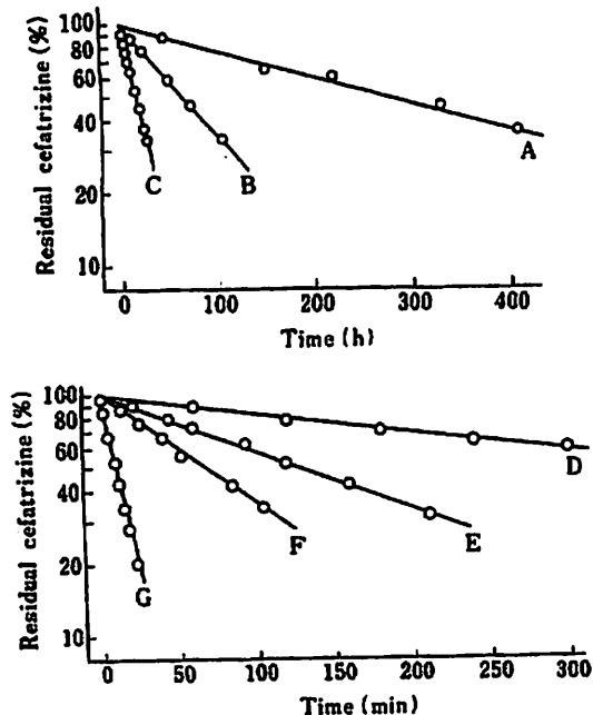
Fig. 1. Apparent First-Order Plots for the Degradation of 5 \times 10^{-3} M Cefatrizine at Various pH Values, 35°C, and an Ionic Strength of 0.5, Determined by HPLC Assay
