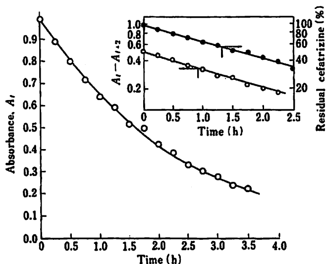
Fig. 6. Time Courses for Primary Amino Group Disappearance during 1 \times 10^{-3} M Cefatrizine Degradation in 0.15 M Phosphate Buffer (pH 7.20) at 35^\circ\text{C} and an Ionic Strength of 0.5
