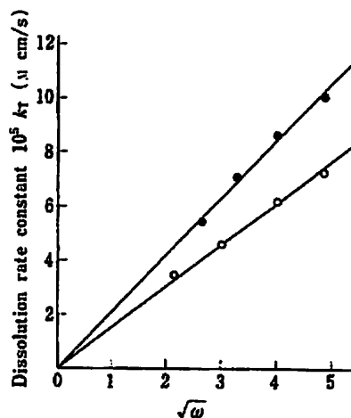
Fig. 9. Effect of Stirring Speed, \sqrt{\omega} , on the Dissolution Rate Constants, k_T , of Cefatrizine Propylene Glycolate (O) and Cefadroxil Monohydrate (●) in 0.5 M KCl at 37°C
