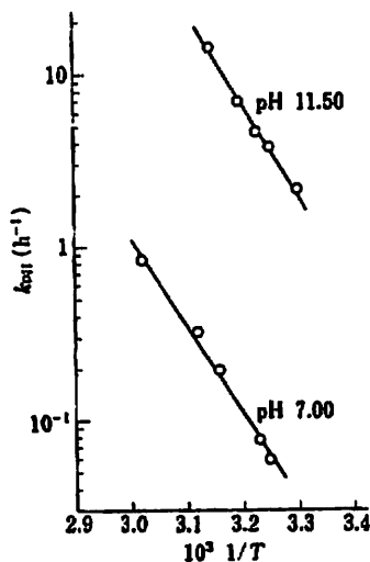
Fig. 7. Arrhenius Plots of the Apparent First-Order Rate Constants, k_{pH} , for Cefatrizine Degradation at pH 7.00 and 11.50, and an Ionic Strength of 0.5.
