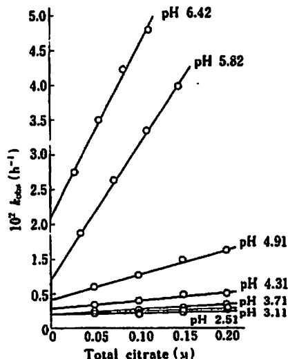
Fig. 2. Plots of Pseudo-First-Order Rate Constant versus Total Citrate Buffer Concentration for Cefatrizine Degradation at Various pH Values, 35°C, and an Ionic Strength of 0.5
