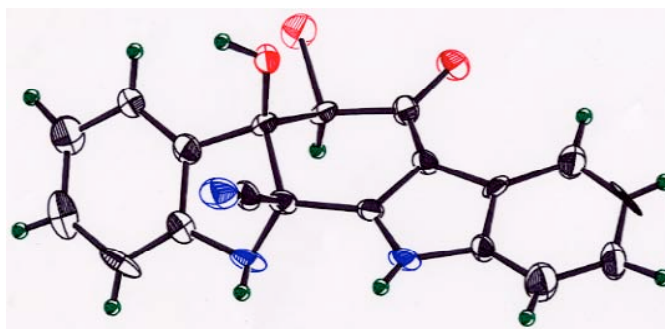
Figure 2. ORTEP Drawing of 11 ( R=0.085 )
