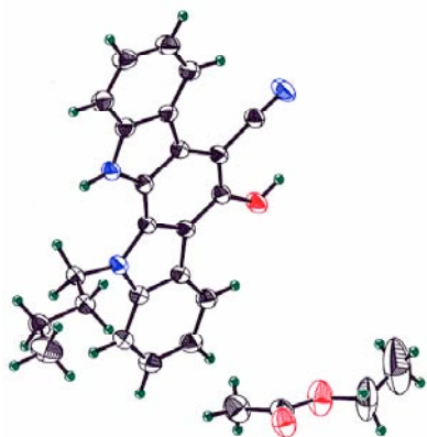
Figure 1. ORTEP Drawing of 9a ( R=0.049 )
