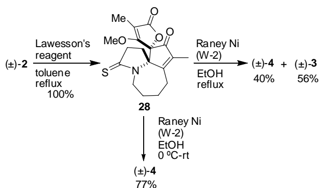
Scheme 8. Synthesis of (±)-4 and (±)-3.
