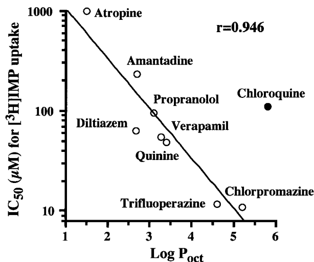
Fig. 8. The Relationship between the IC_{50} for [^3H]IMP Uptake and the \log P_{oct} for Basic Drugs
