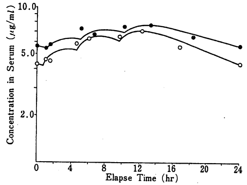
Fig. 2 The patterns of the diurnal oscillations of the CBZ serum levels with lag time The measured levels of Case K.M. and S.Y. are represented by \bullet and \circ
