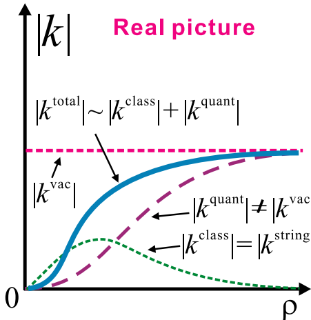
FIG. 3 (color online). The real qualitative behavior of the density of monopoles around the QCD string.
