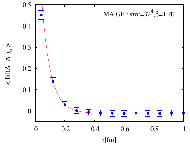
FIG. 6 (color online). The correlation between the monopole density |k_\mu| and the operator A^+A^- in the MA gauge. The solid line denotes the best exponential fit by the function (49) with the best fit parameters given in Table I.
