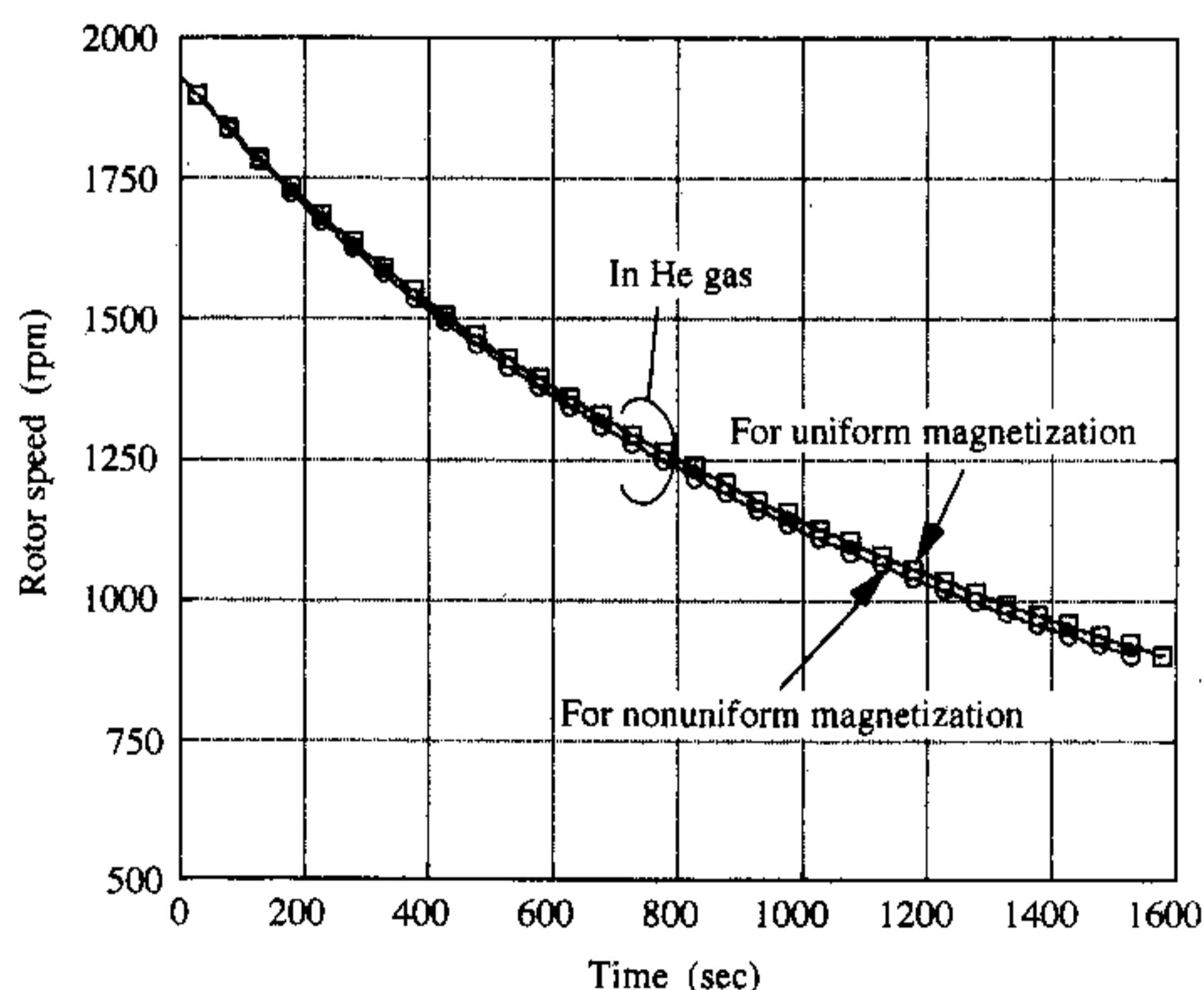
Fig. 6. Deceleration characteristics of the rotor.
