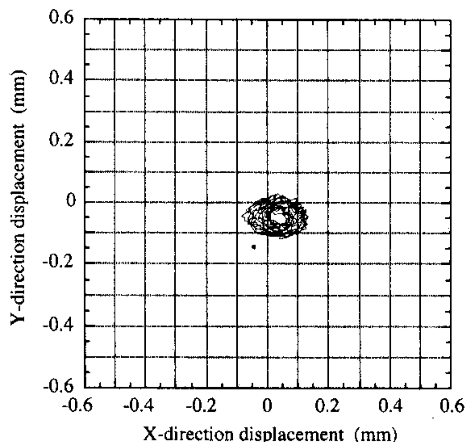
Fig. 4. Vibration characteristics with the nonuniformity in rotor.
