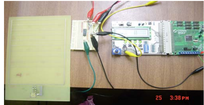
Figure 7: Microcontroller based low cost sensing system
