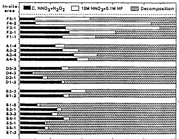
Percentage of stepwise leaching of Pu in soil
