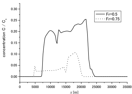
Figure 5 Ground scalar concentration for Fr = 0.5 and 0.75
