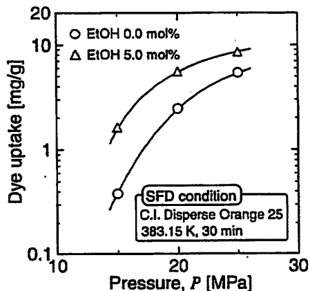
Fig.7 Relationship between dye uptake and dyeing pressure.
