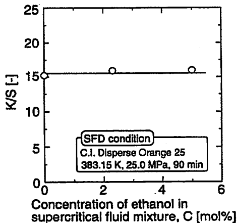
Fig.9 Relationship between dye uptake and entrainer concentration.
