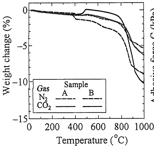
Fig.6 Result of TG of flyash specimen
