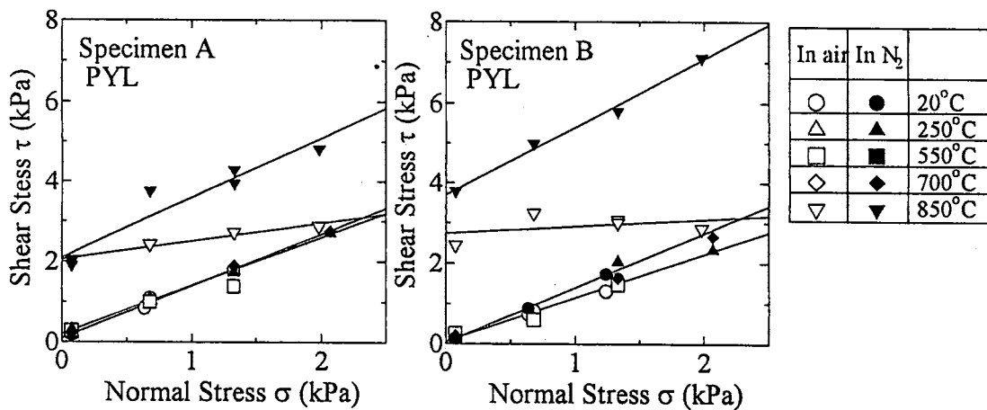
Fig.2 Powder yield loci of specimen
