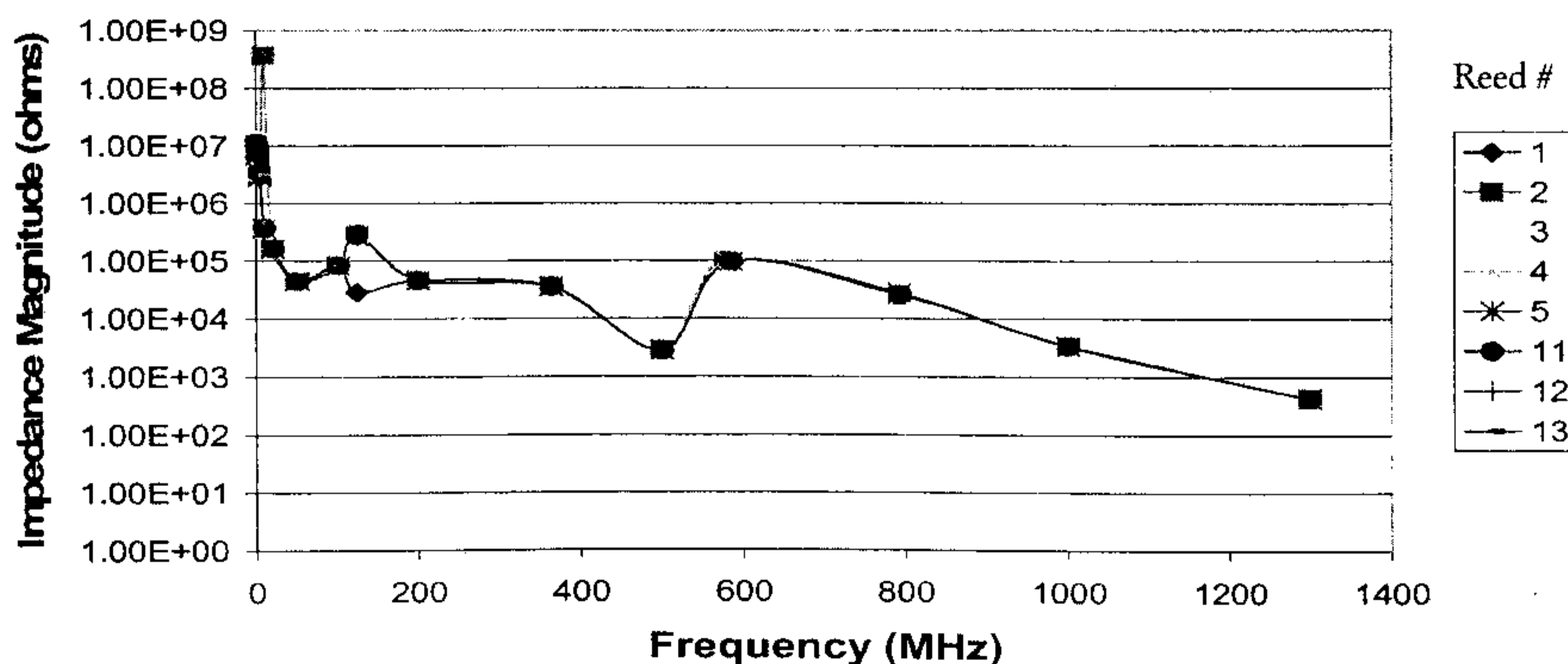
Fig. 5: Magnitude Response of Sensor
