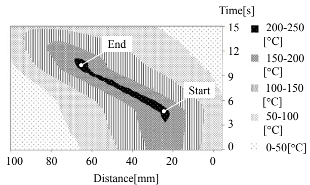
Fig.6 Temperature distributions
