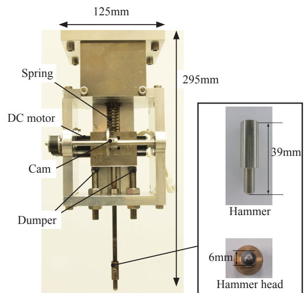
Fig.3 Hammering unit
