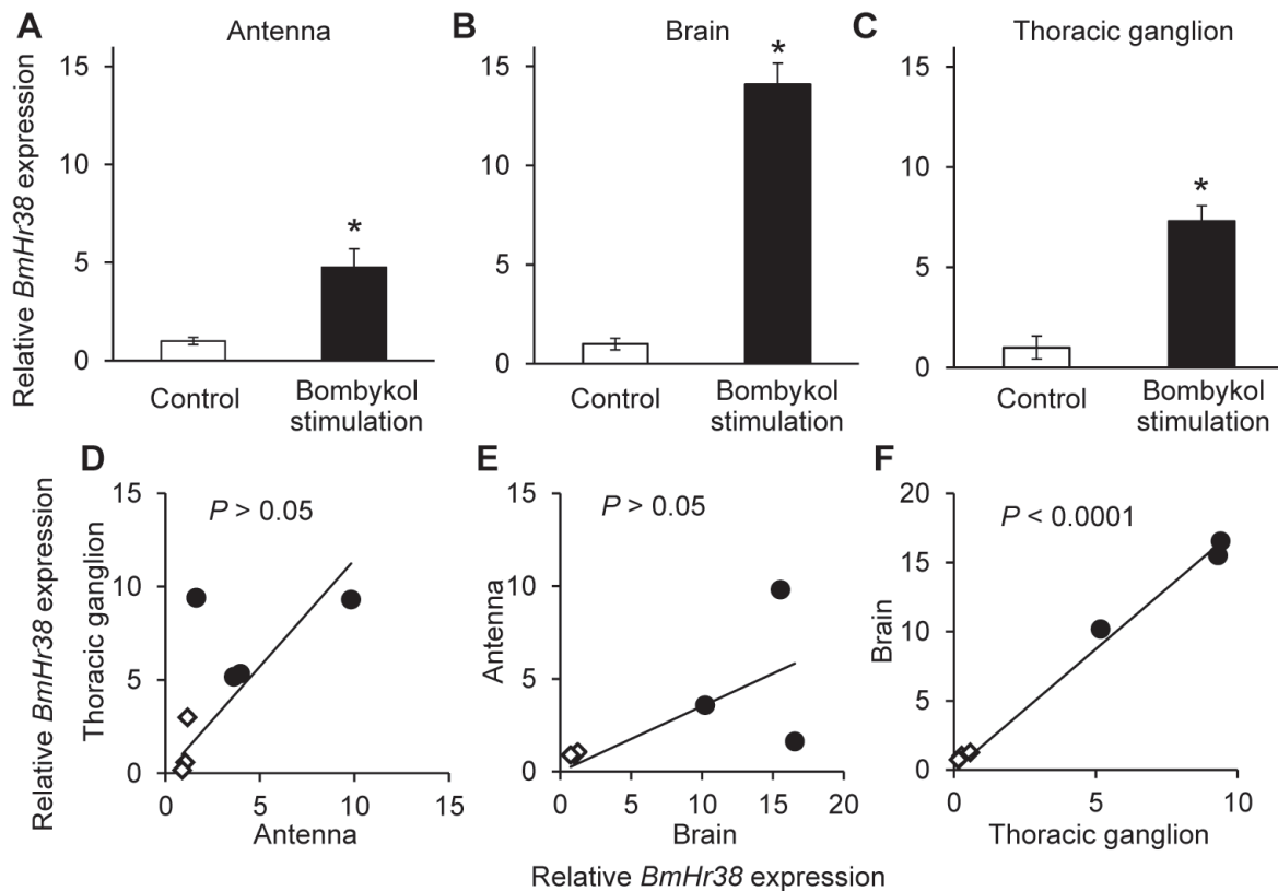
Fig. 1. QRT-PCR analysis of BmHr38 expression in response to sex pheromone stimulation in the antennae, brains, and thoracic ganglia. (A–C) Relative expression levels of BmHr38 in the antennae (A), brains (B), and thoracic ganglia (C) of control (no stimulation) or bombykol-stimulated male silkmoths. n = 3 (brains) or 4 (antennae and thoracic ganglia), each. *: P < 0.05 , U -test. (D–F) Regression analysis of BmHr38 expression levels between tissues. Open squares and filled circles indicate control and bombykol-stimulated samples, respectively.
