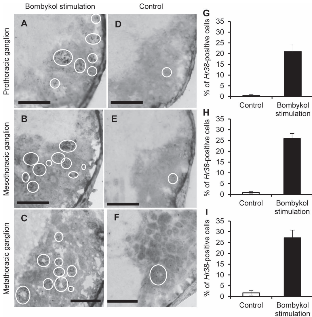
Fig. 2. Expression pattern of BmHr38 in the thoracic ganglia revealed by in situ hybridization. (A–F) Expression pattern of BmHr38 in the prothoracic (A, D), mesothoracic (B, E), and metathoracic (C, F) ganglia with (A–C) or without (D–F) bombykol-stimulation. White circles indicate BmHr38 -expressing cells. Scale bars, 50 \mu m. (G–I) Proportion of BmHr38 -positive cells in each ganglion. n = 4 –7, each.
