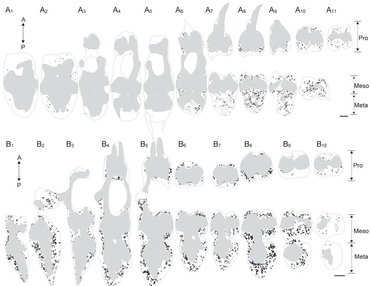
Fig. 3. Schematic drawings of BmHr38 expression pattern in the thoracic ganglia of male moths stimulated with bombykol. Schematic summaries of expression pattern of BmHr38 in two representative thoracic ganglia (A and B) of bombykol-stimulated silkmoths. The sections (A 1–11 and B 1–10 ) are numbered and placed from dorsal to ventral. Signals and neuropilar area are shown in black and gray, respectively.
