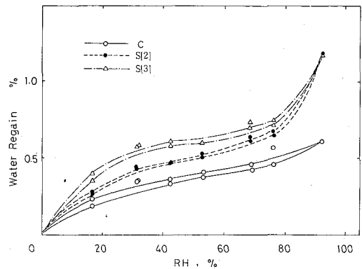
Fig. 3 Relationship between relative humidity and water regain.
