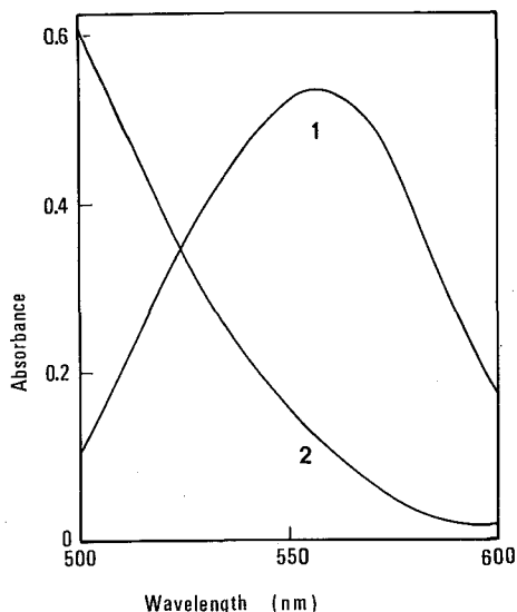
Fig. 1. Absorption curves of scandium-SMXB complex in a 25 ml aqueous solution containing 20 \mu\text{g} of scandium and 3 ml of 0.05% SMXB solution at pH 2.7 (1) and of the reagent blank (2). The absorbances were measured against the reagent blank (1) and water (2) as references.
