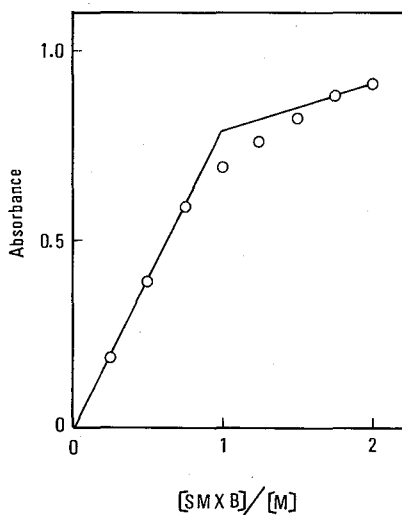
Fig. 6. The mole ratio method examined with a 25 ml aqueous solution containing a constant amount of scandium, 7.1 \times 10^{-7} M, and various amounts of SMXB at pH 2.7. The absorbance was measured at 559 nm against a reagent blank as a reference.
