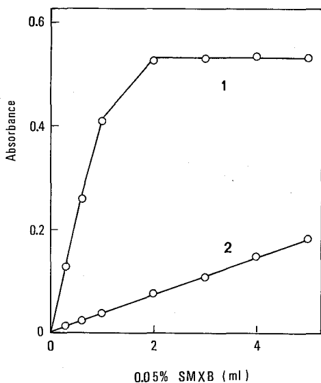
Fig. 3. Effect of SMXB concentration on the absorbance of scandium-SMXB complex (1) and the reagent blank (2), examined with a 25 ml aqueous solution containing 20 \mu\text{g} of scandium at pH 2.7. The absorbances were measured at 559 nm against the reagent blank (1) and water (2) as references.
