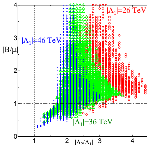
Figure 1: The ratio of |B| to |\mu| required by the radiative symmetry breaking conditions.
