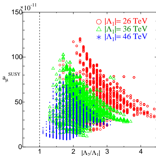
Figure 4: The predicted value of the AMM of a muon in the parameter space where the EDM bounds and the phenomenological constraints are satisfied.
