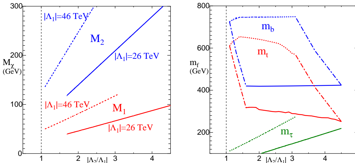
Figure 2: Mass spectrum of the low lying superpartners for various values of |\Lambda_{1,2}| . The left panel shows the gaugino masses related to charginos and neutralinos. The right panel shows the third generation sfermion masses. In each panel the solid lines correspond to |\Lambda_1| = 26 TeV and the dotted lines correspond to |\Lambda_1| = 46 TeV.
