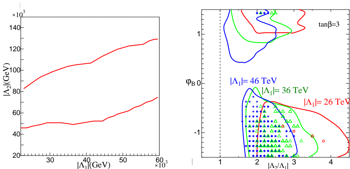
Figure 3: The left panel shows the allowed region in the (|\Lambda_1|, |\Lambda_2|) plane which satisfies both the EDM constraints and the phenomenological conditions given in the text. The right panel shows the allowed region of \phi_B (= -\phi_\mu) for the same constraints. In both panel the region surrounded by the curves are allowed.
