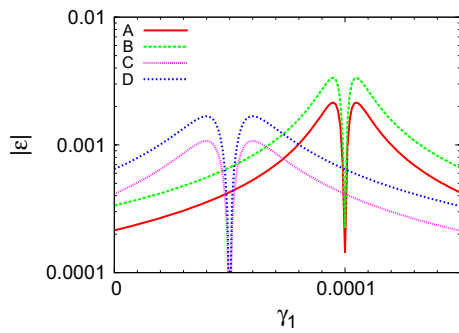
Fig. 1 CP asymmetry as a function of \gamma_1 for typical values of (|y_1|, |h_{\alpha 1}|) . In each case, these parameters are fixed as A( 10^{-5}, 4 \times 10^{-4} ), B( 10^{-5}, 5 \times 10^{-4} ), C( 2 \times 10^{-5}, 4 \times 10^{-4} ), and D( 2 \times 10^{-5}, 5 \times 10^{-4} ). Other relevant parameters are taken to be \tilde{\gamma}_1 = 0.1, \tilde{y}_1 = 10^{-8}, M_1 = \langle S \rangle = 2 \text{ TeV} and M_\eta = 1 \text{ TeV}
