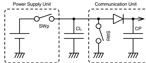
Figure 2. Circuit architecture of data communication and power supply unit of TextileNet.
