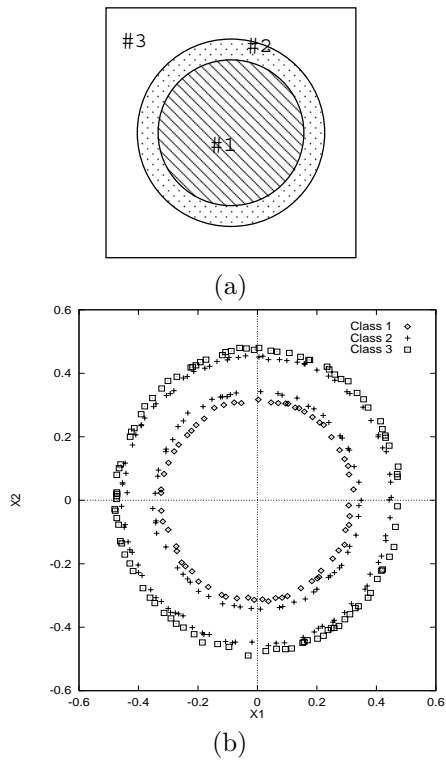
Figure 4: (a) Concept of class data distribution. (b) Selected boundary data by proposed method
