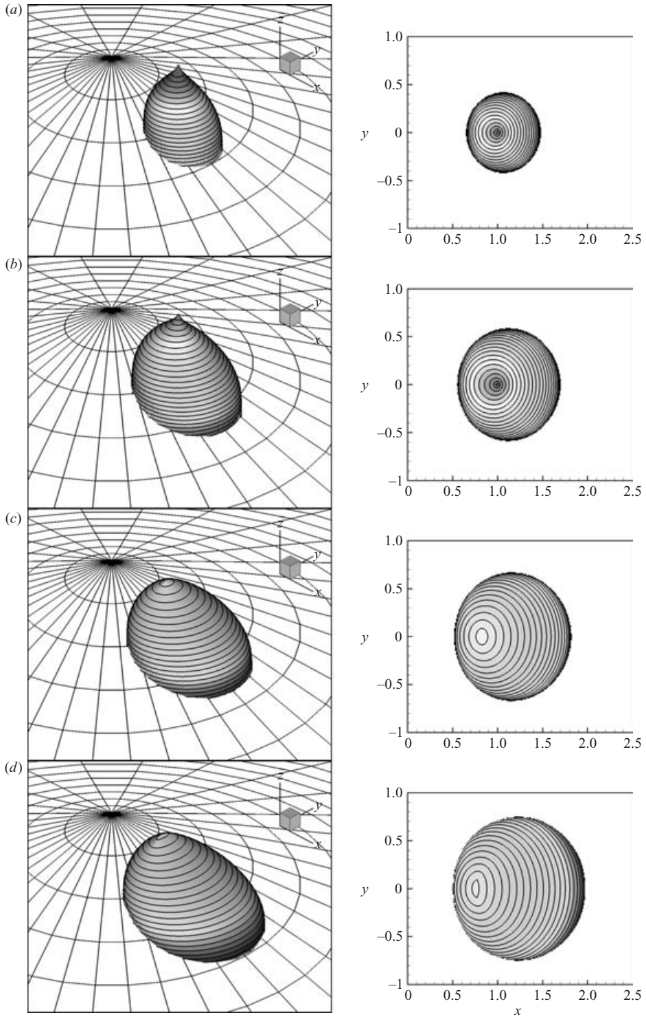
FIGURE 18. Mud spreading from a hillside for V_0 = 1 and Q_0 = 1 . (a) t = 0.5 , (b) 1, (c) 1.5, (d) 2.0. The source is at x_s = 1 , y_s = 0 . Mud is discharged until t = 1 . In the right-hand column, the contour lines of the free-surface height are plotted with the interval \Delta h = 0.1 . The highest contour is (a) h = 0.7 , (b) h = 0.8 , (c) h = 0.2 , (d) h = 0.1 , respectively.
