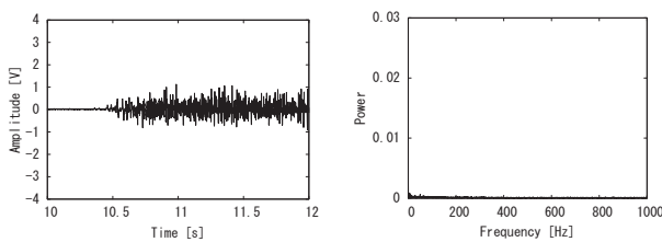
(a) Waveform (without arm force before 10.5 s and with arm force after 10.5 s). (b) Spectrum (without arm force).
