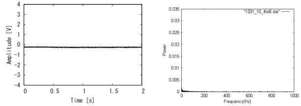
(a) Waveform (without arm force). (b) Spectrum (without arm force).
