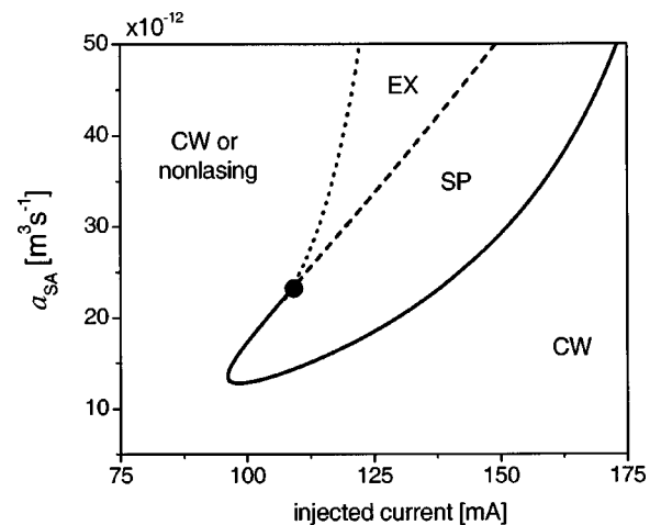
FIG. 6. The bifurcation diagram in the plane of saturable absorber differential gain coefficient vs injected current for a laser with a cavity length of 650 \mu\text{m} and a saturable absorber thickness of 2 nm. The carrier lifetimes in the active region and in the saturable absorber are 2 and 0.5 ns, respectively. The other parameters are as in Table I. The laser behaviour in the different regions is denoted by excitable (EX), self-pulsating (SP), and CW or nonlasing. The solid line represents a Hopf-bifurcation line.
