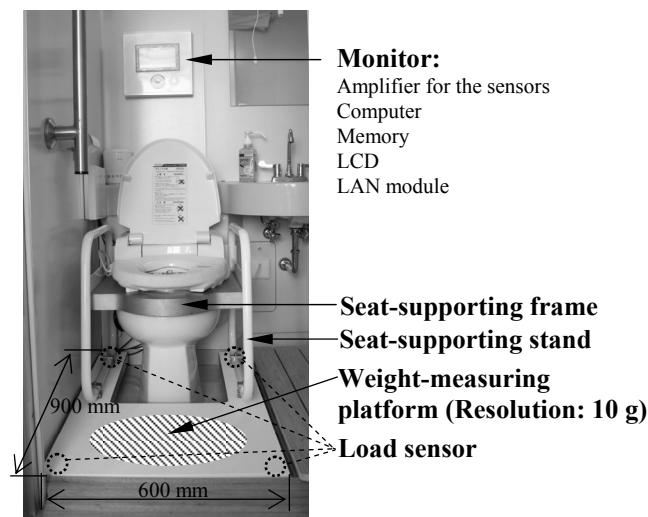
Fig. 2. Details of the sensor system installed at the toilet space which can measure the body and excretion weight.
