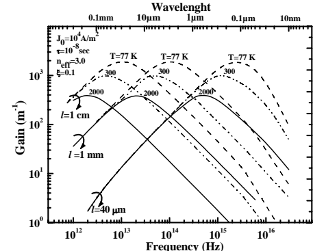
Fig. 5. The gain peak variation with the EM frequency by the CEW-Model.
