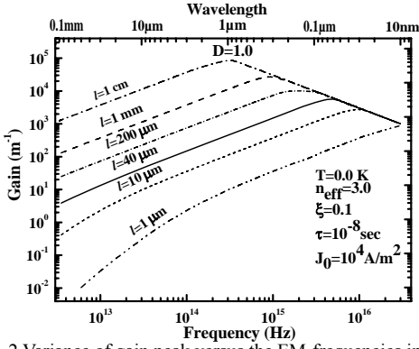
Fig. 2 Variance of gain peak versus the EM-frequencies in CEW-Model.
