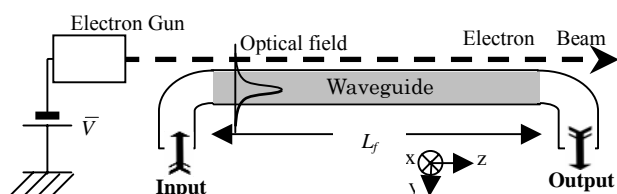
Fig.1 Illustration scheme of EM- wave amplifier.
