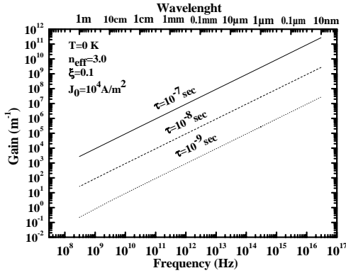
Fig. 3. The gain peak variation with the EM frequency by the LE-Model.
