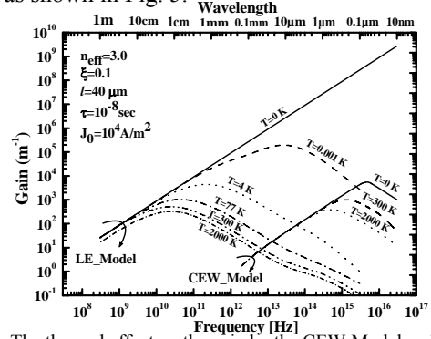
Fig. 4. The thermal effect on the gain by the CEW-Model and LE-Model.
