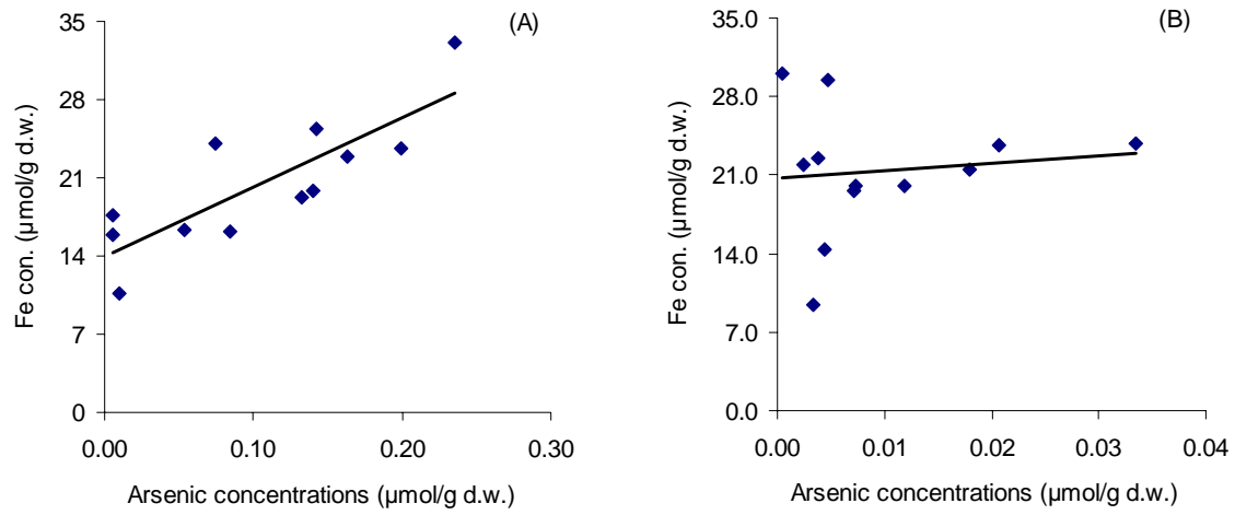
Fig. 4: Correlation between arsenic and iron concentrations in of Salvinia natans L. exposed to arsenate (A) and DMAA (B).
