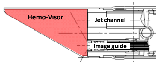
Fig. 3 Detail of the endoscope tip
