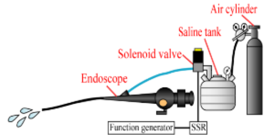
Fig. 4 Outline of the saline discharge system
