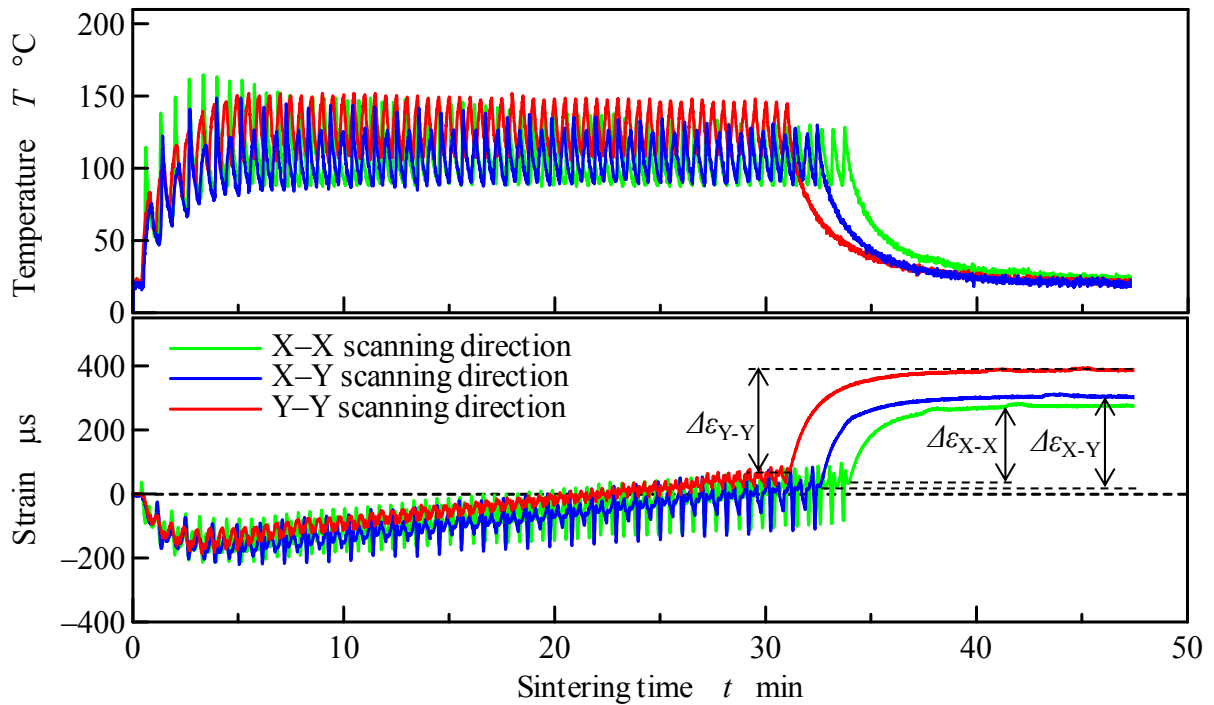
Fig. 7 Temperature and strain history during sintering process
