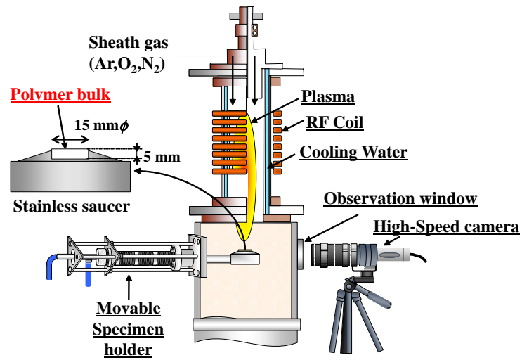
Figure 1. ICP torch and chamber.
