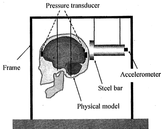
Fig.2 Experimental apparatus
