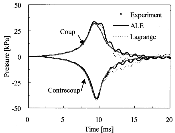
Fig.3 Comparison of the pressure response in the simulations with the occipital impact experiment in case of 5kg mass steel bar and 1.5m/s velocity
