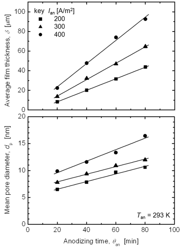
Fig. 3. Effect of current density and processing time on average film thickness and pore diameter of anodized aluminum ( T_{an} = 293 \text{ K} ).
