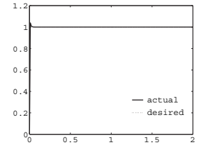
(e) Trajectory of \tilde{f}_3
