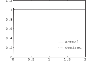
(c) Trajectory of \tilde{f}_1
