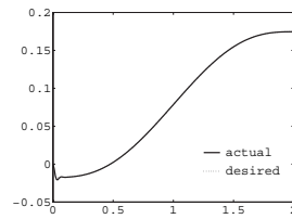
(b) Trajectory of \phi
