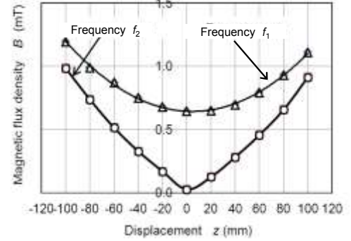
(c) Magnetic flux density along z -axis at two resonance frequencies
