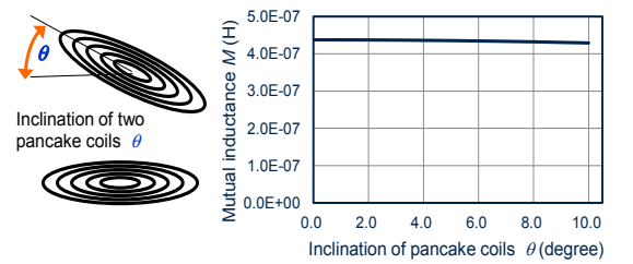
Fig. 10 Change of mutual inductance on inclination of pancake coils.
