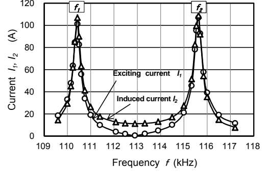
(a) Currents of exciting I_1 and induced currents I_2
