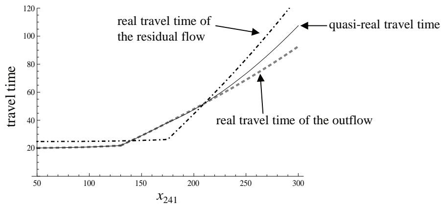
Figure 7: The two real travel times and quasi-real travel time
