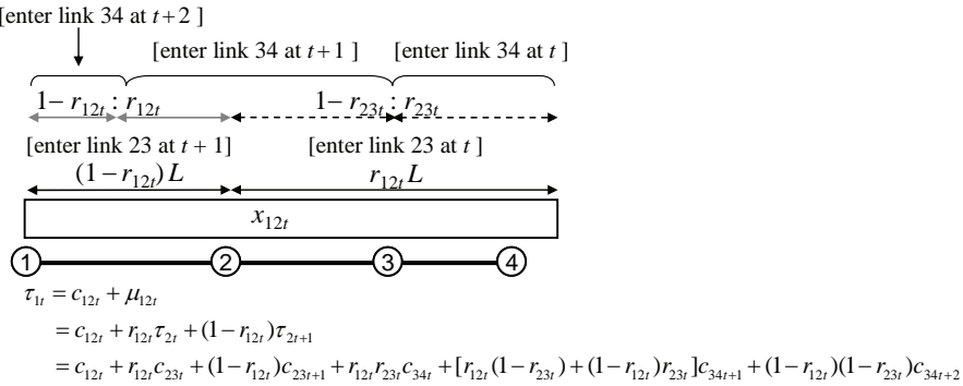
Figure 3. Quasi-real travel time
