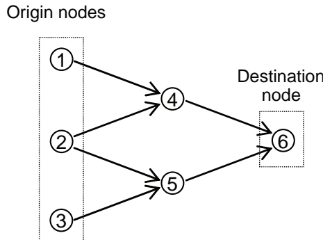
Figure 4: Example network
