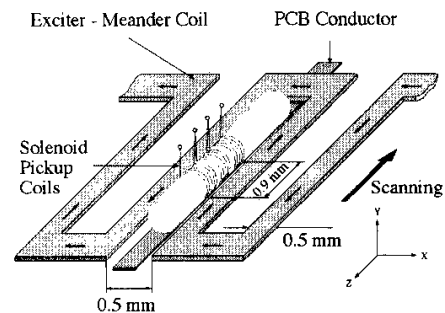
Fig. 1. ECT sensor for the inspection of printed circuit board.
