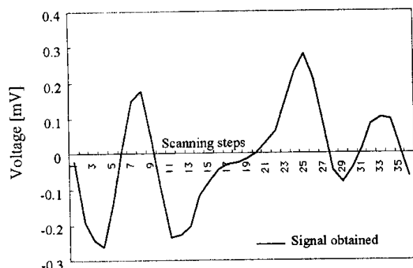
Fig. 5. Resultant pattern signal.
