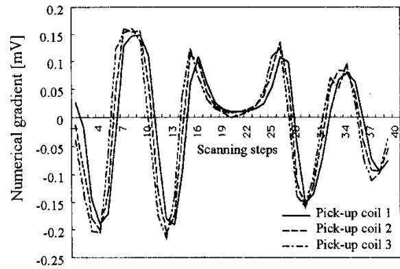
Fig. 4. Numerical gradients of the subsignals.
