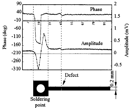
Fig. 2. Amplitude and phase obtained from the inspection of one conductor and soldering point.
