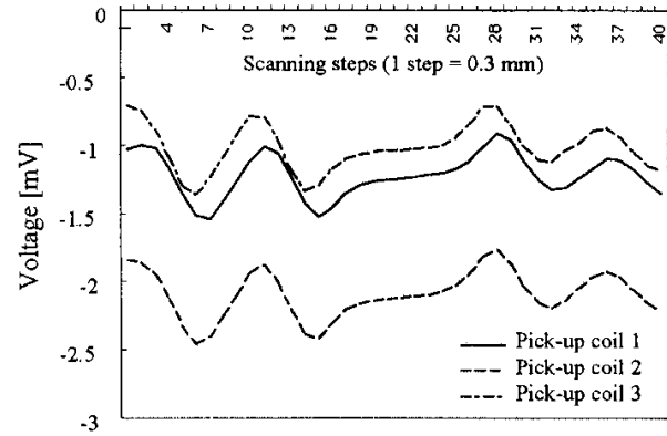
Fig. 3. Subsignals obtained from each pick-up coil (amplitude data).
