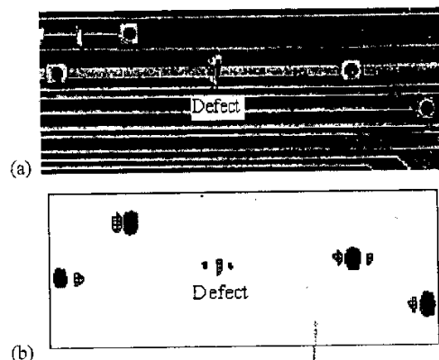
Fig. 6. Inspection results (a) PCB model, (b) image using amplitude data.
