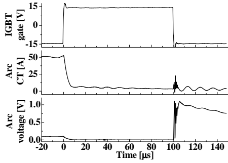
(a) successful interruption
