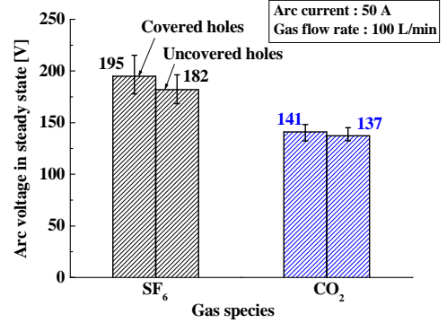
Fig. 14. Averaged arc voltage measured in steady state.
