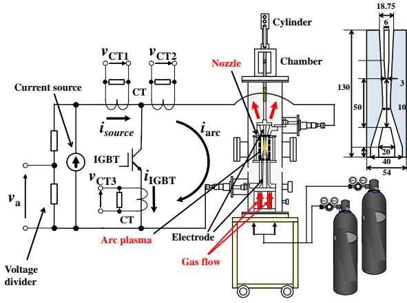
Fig. 4. Experimental setup for gas-blast arc experiment.
