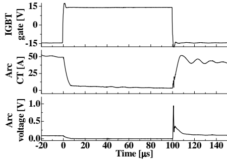
(b) Interruption failure
