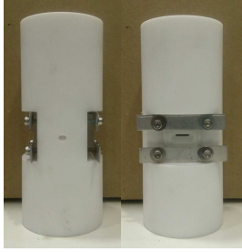
Fig. 5. Gas-blast nozzles for the experiments
