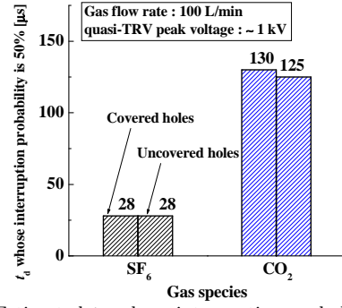
Fig. 13. Estimated t_d whose interruption probability is 50%.
