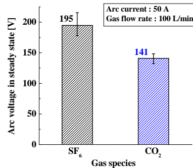
Fig. 10. Averaged arc voltage measured in steady state.
