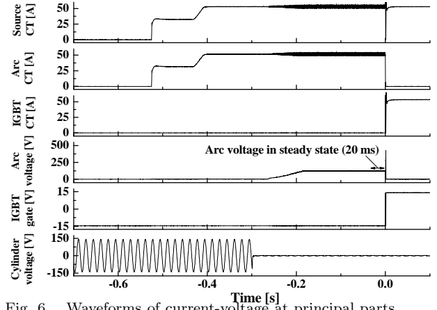
Fig. 6. Waveforms of current-voltage at principal parts.
