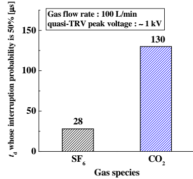
Fig. 9. Estimated t_d for 50% of interruption probability.
