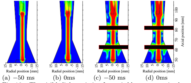
Fig. 16. The visible light emission from air blast arc sustained in the nozzle. (a) without holes at t = -50 ms and (b) without holes at t = 0 ms. (c) with holes covered by plates at t = -50 ms and (d) with holes covered by plates at t = 0 ms.
