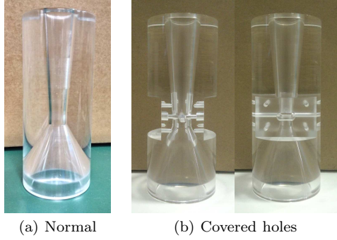
Fig. 15. Gas-blast nozzles for the high speed video camera observation.
