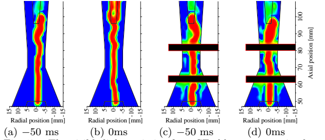
Fig. 17. The visible light emission from SF_6 blast arc sustained in the nozzle. (a) without holes at t = -50 ms and (b) without holes at t = 0 ms. (c) with holes covered by plates at t = -50 ms and (d) with holes covered by plates at t = 0 ms.
