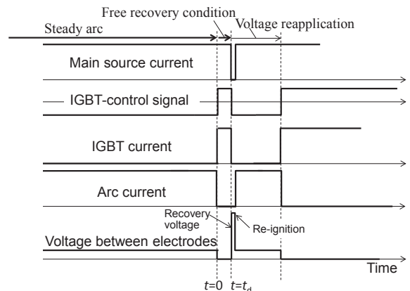
Fig. 3. Conceptual current and voltage behaviors in case of interruption failure after quasi transient recovery voltage application.
