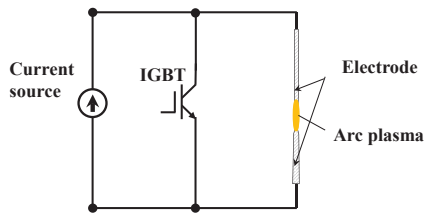
Fig. 1. Conceptual circuit for investigation of decaying arcs and arc re-ignition.
