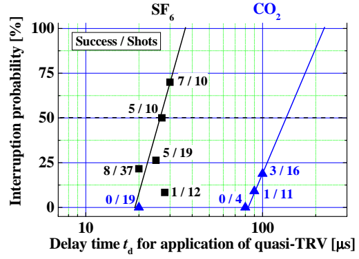
Fig. 8. Dependence of successful interruption probability on delay time t_d for quasi-TRV application, in cases of the nozzle with holes covered by plates.
