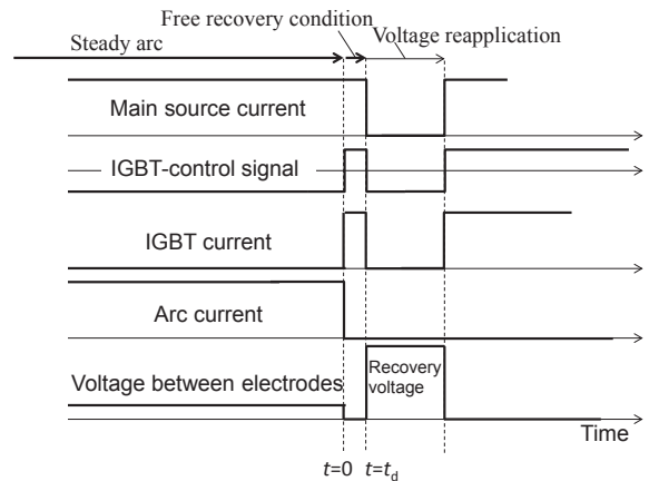
Fig. 2. Conceptual current and voltage behaviors in case of success of arc interruption after quasi transient recovery voltage application.
