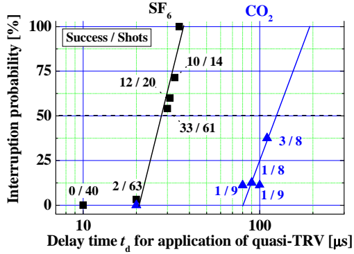
Fig. 12. Dependence of percentages of successful interruption on delay time t_d for quasi-TRV application, in the cases of the nozzle with uncovered holes.
