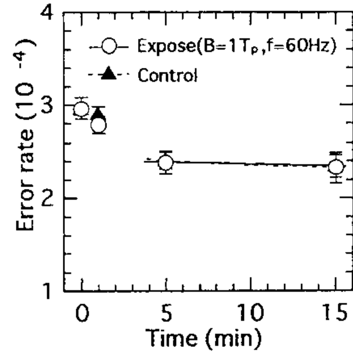
Fig.6 Influences on the error rate of DNA synthesis when klenow is used.
