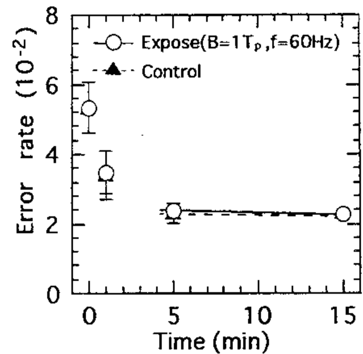
Fig.7 Influences on the error rate of DNA synthesis when exo(-) klenow is used.
